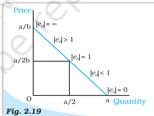
Fig. 2.19 Elasticity along a Linear Demand Curve. Price elasticity of demand is different at different points on the linear demand curve.
