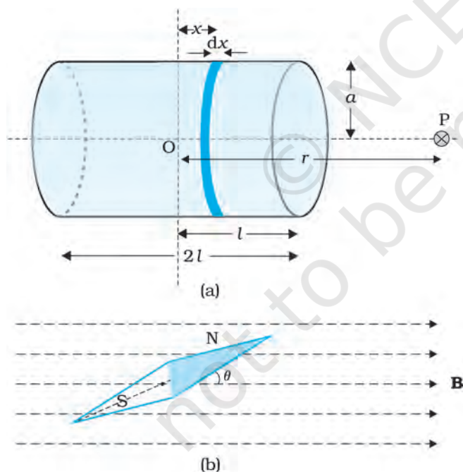
FIGURE 5.3 Calculation of (a) The axial field of a finite solenoid in order to demonstrate its similarity to that of a bar magnet. (b) A magnetic needle in a uniform magnetic field B . The arrangement may be used to determine either B or the magnetic moment m of the needle.
